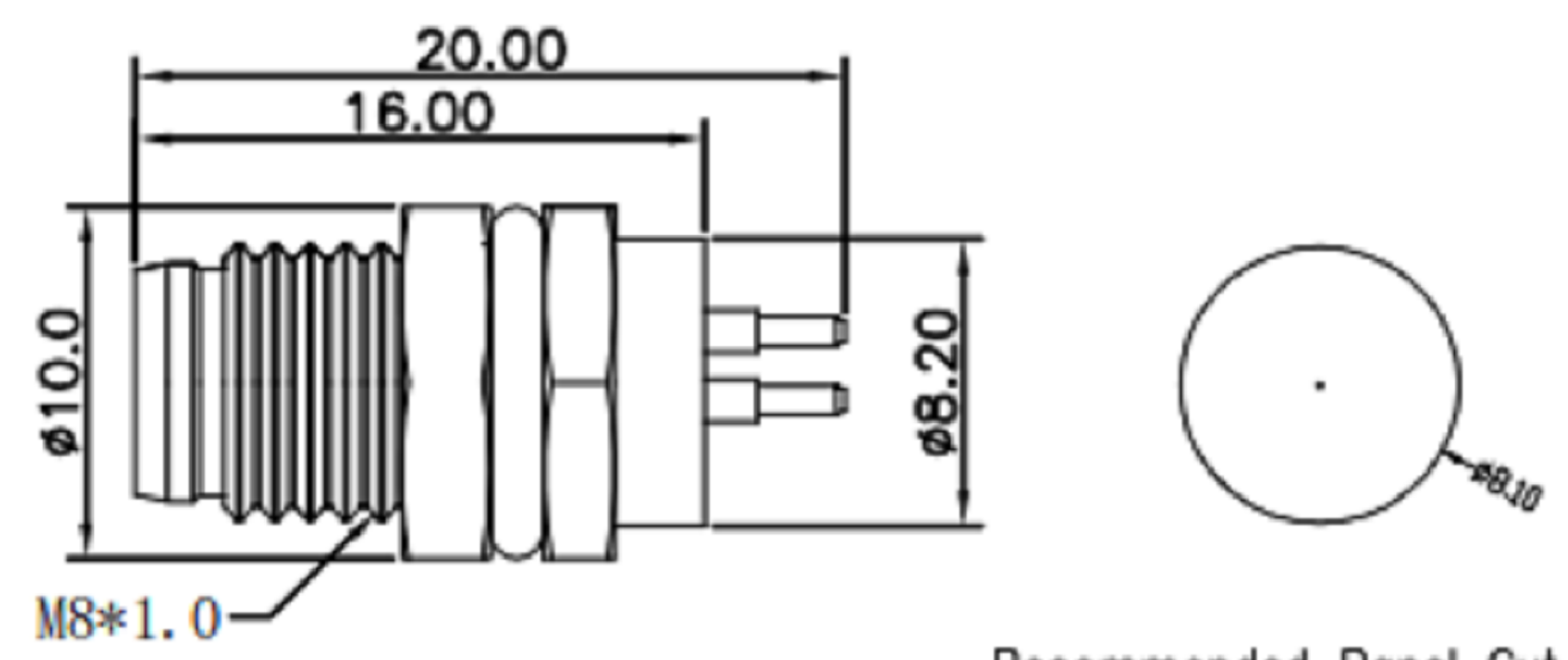
Scale drawing/尺寸图
