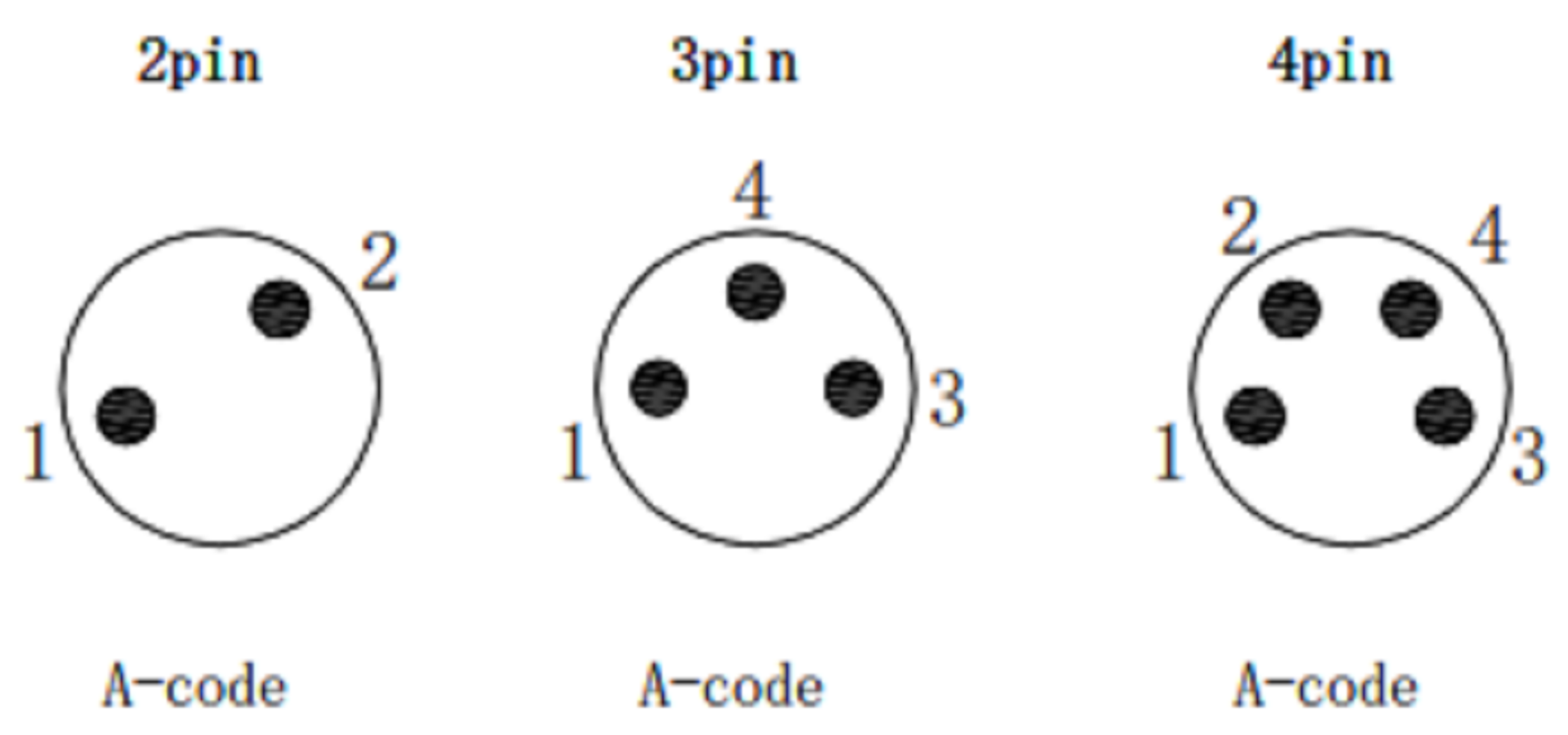
Pin assignment front view/针位分布前视图
